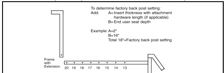
Figure 6.1 - Frame Depth Diagram
